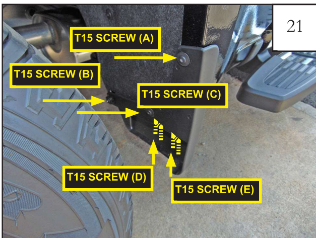
Locate the mud flap in front of the rear wheel. Remove (5) factory installed T15 screws. Note that T15 screws labeled (A) and (C) will be re-used to install the flare. You may discard (B), (D), and (E).
