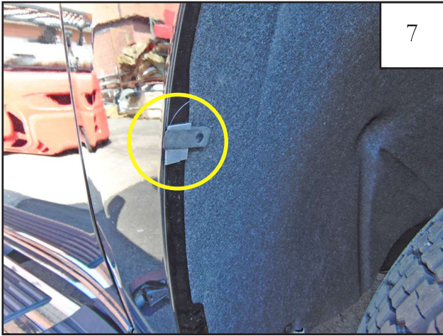
Install supplied Tab (MT1-0034) over the rear location marked in Step 6. Install a Clip (CL1-0009) as indicated on top of the protective film.
