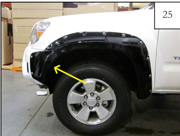
Make sure bumper piece is aligned with the style line. Install supplied 20mm hex screw (SW1-0036) into factory hole on front bumper and tighten.
